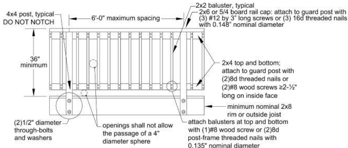
Figure 24. Example Guard Detail.
