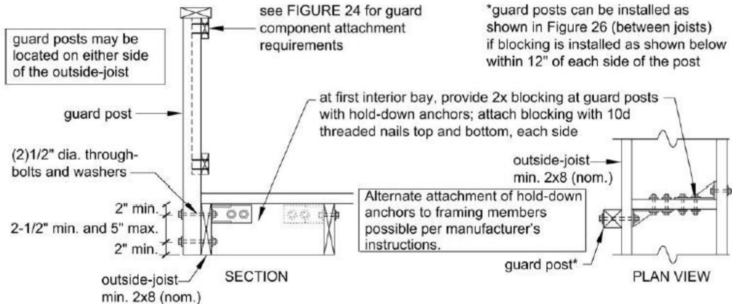
Figure 25. Guard Post to Outside-Joist Example.
