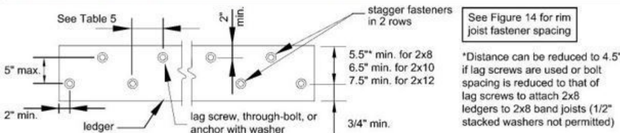
Figure 19. Ledger Board Fastener Spacing and Clearances.
