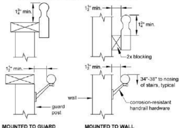
Figure 32B. Handrail Grip Size.
