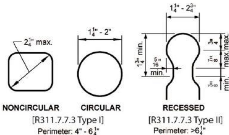
Figure 32B. Handrail Grip Size.
