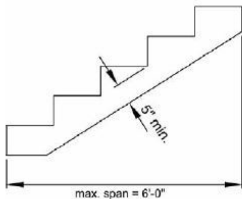
CUT STRINGER
